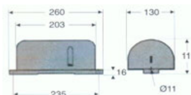
Vibrator V-20
