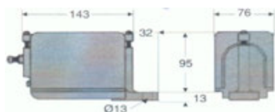
Vibrator V-4
